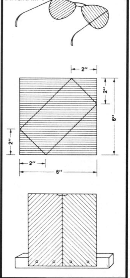
Commercially made 3-D glasses have a diagonal orientation. They require that filters in the projection system be specially cut.
